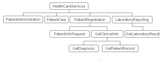
Figure 3: An example of Service Functionality Ontology
