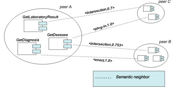
Figure 6: An example of semantic neighbors for the peer A
